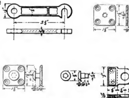
Figs. 2897-2906. Dog, Hasp and Seal Plate for Doors and Drawers.
